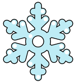
SNOWFLAKE
